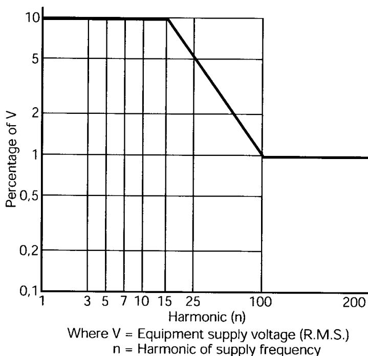
Fig. 1.22.1 Harmonic/test voltage for conducted low frequency interference
